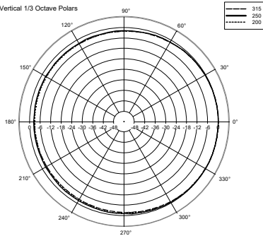
Vertical 1/3 Octave Polars
